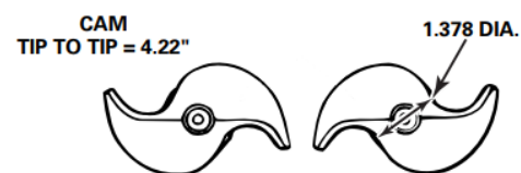
16.5" Q CAMSHAFT (1.5" DIA.-10 OR 28 SPLINES)
