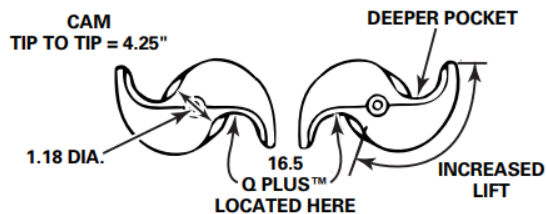
16.5" Q PLUS™ CAMSHAFT (1.5" DIA.-28 SPLINES)
